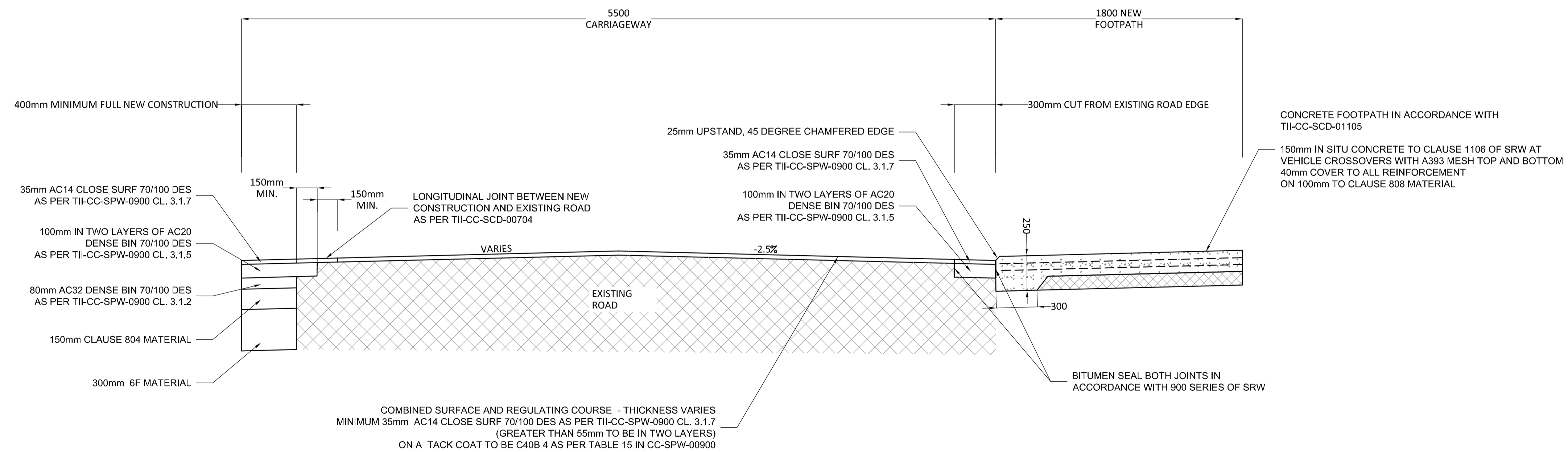
SECTION B -B. (VEHICLE CROSSOVERS) SCALE 1:20
